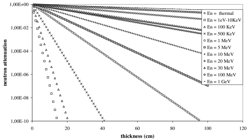
Figure1. Neutron attenuation in polyethylene moderator
